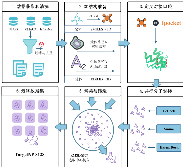
Fig. 1. The construction process of the TargetNP-8128 dataset.
