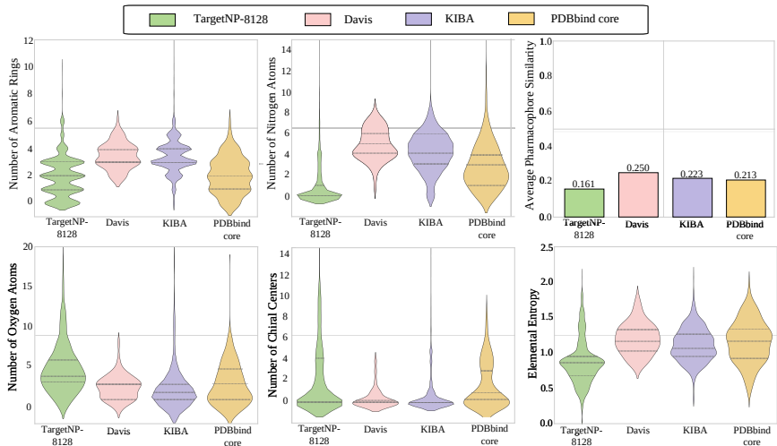
Fig. 4. Comparison of four drug datasets in terms of key molecular characteristics.
